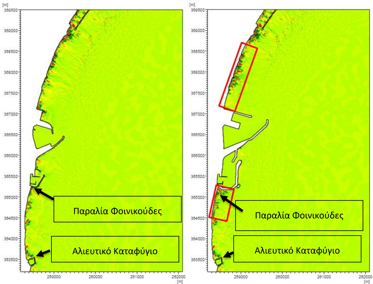
Figure 10-2. Weighted annual rate of sea bottom change and influence zones (depicted with red rectangles); Left panel: DN, Right Panel: W2.
